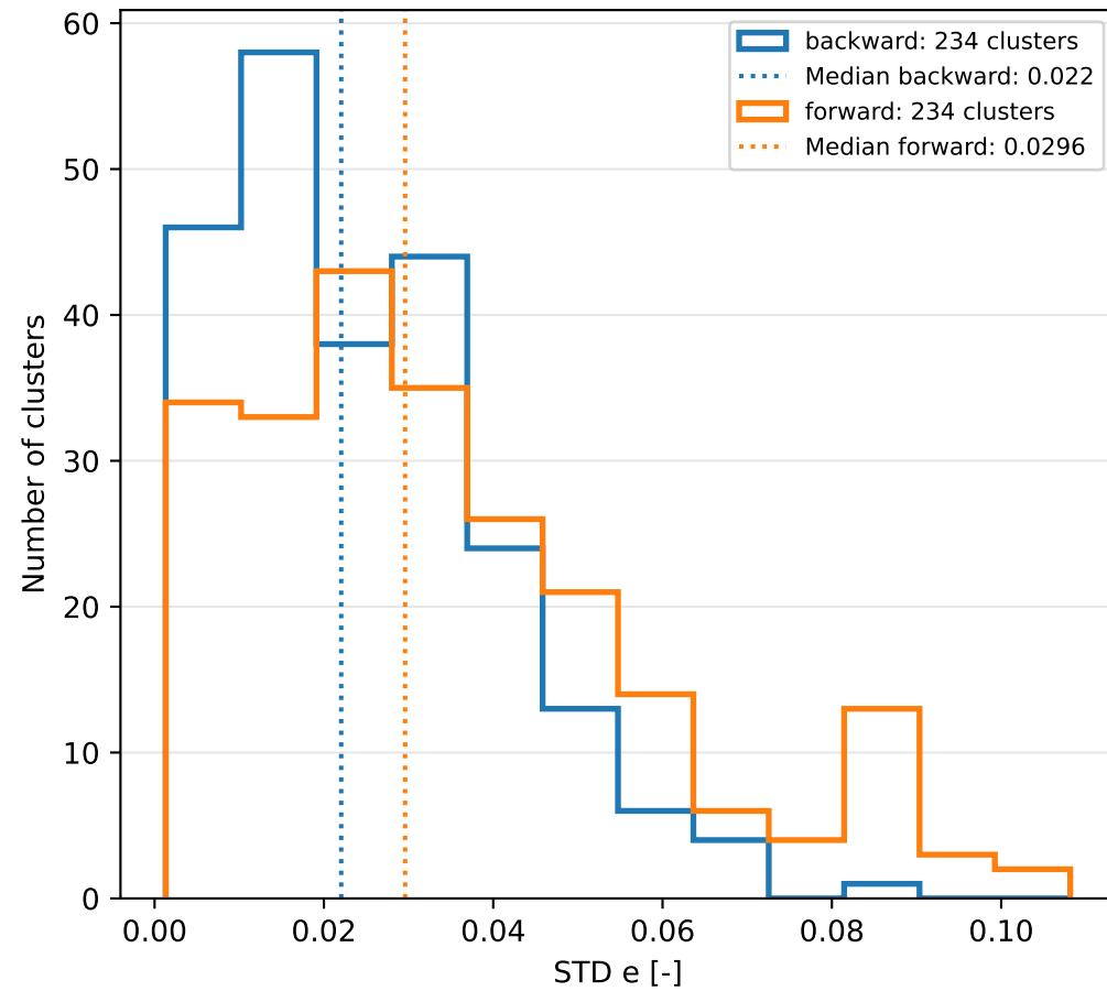
K=234 | Within-cluster STD distributions | Each cluster counts once
